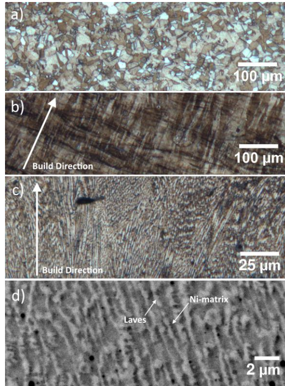
Fig. 2 OM images of etched a) equiaxed substrate grains, b) elongated deposition grains, c) cellular dendritic subgrain within deposition and d) SEM image (BSE) of dendrite (Ni-matrix) and interdendritic (Laves) regions
