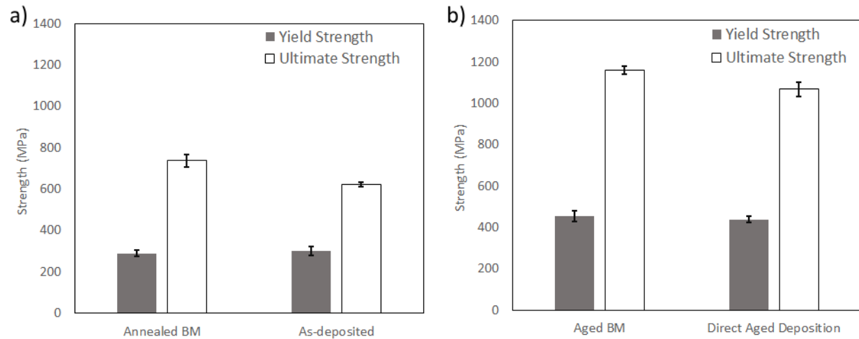
Fig. 9 Tensile test results for a) annealed base metal (BM) and as-deposited alloy 718 with standard error bars and b) after aging heat treatments for BM and deposited alloy 718 with standard error bars
