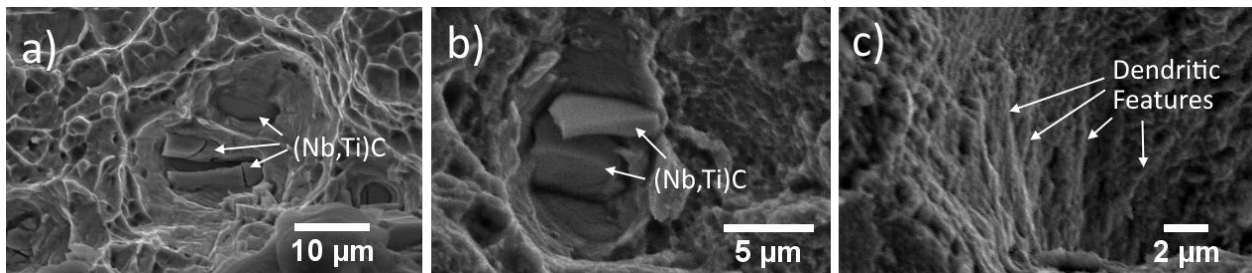
Fig. 11 Fracture surface SEM images of a) (Nb,Ti)C in an aged base metal specimen, b) (Nb,Ti)C in an aged deposition specimen, and c) dendritic features on the fracture surface of an aged deposition specimen
