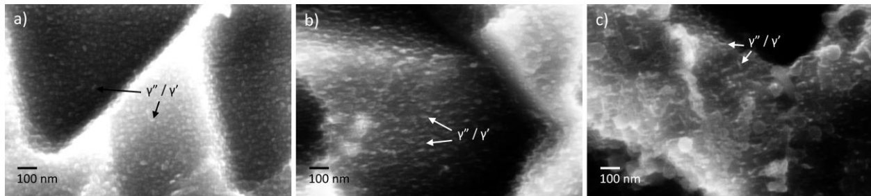
Fig. 6 FE-SEM using the Zeiss InLens SE detector of \gamma'' and \gamma' precipitates in an etched a) substrate alloy 718 after aging, b) HAZ after deposition and aging, and c) deposition after direct aging
