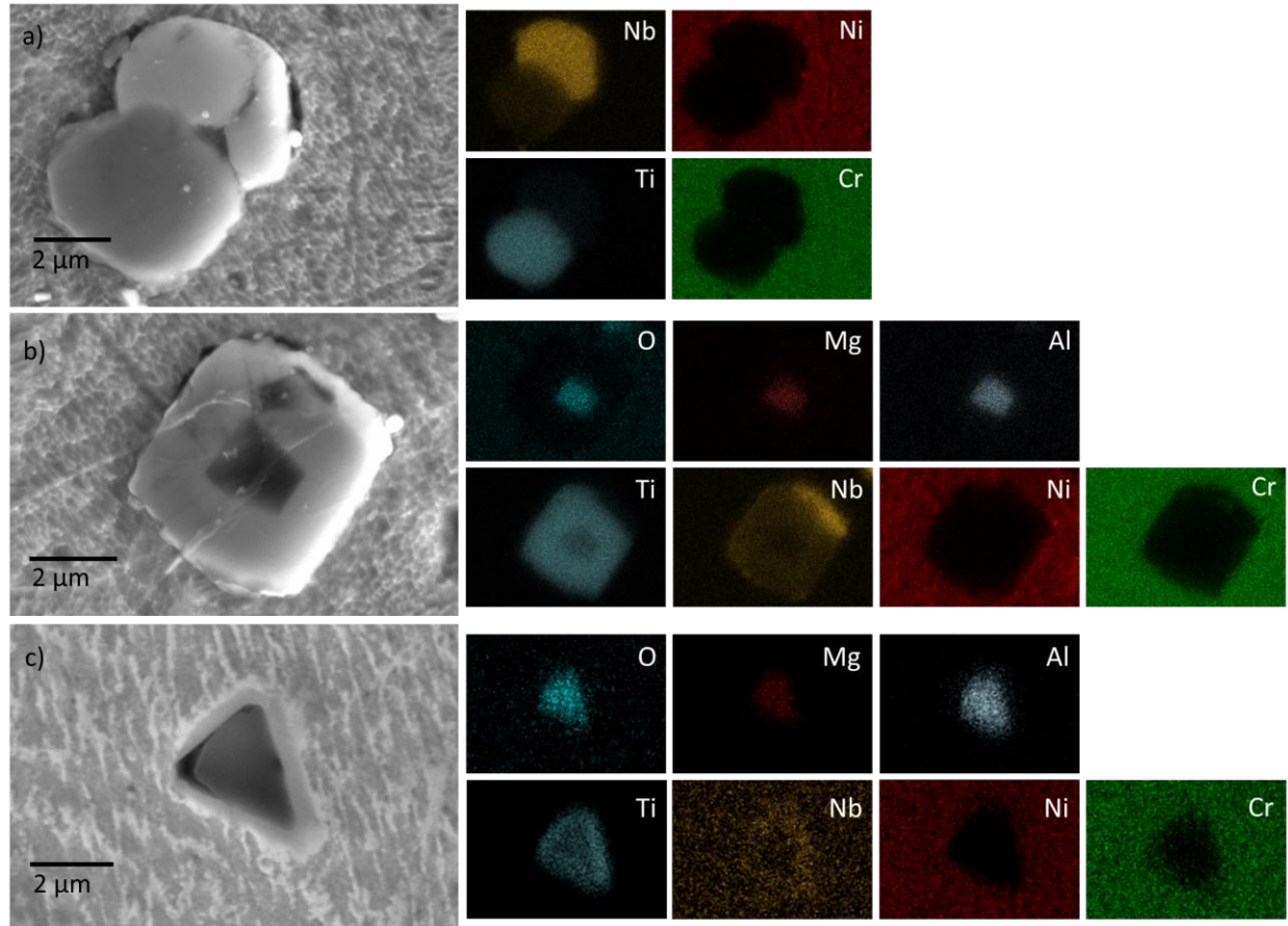
Fig. 5 Etched SEM images of aged substrate alloy 718 with a) adjacent (Nb,Ti)C and (Ti,Nb)CN, b) substrate carbide with (Mg,Al)O core, (Ti,Nb)CN shell, and sliver of (Nb,Ti)C, and c) deposition carbide with (Mg,Al)O core and (Ti,Nb)CN shell
