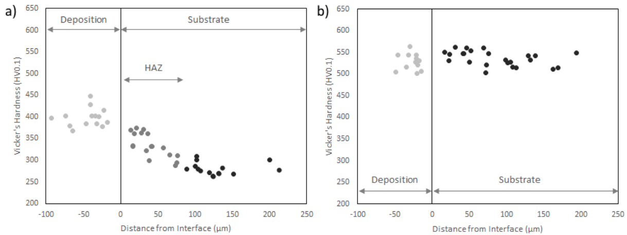
Fig. 7 Alloy 718 depositions on solution annealed alloy 718 with a) no post-ESD heat treatment and b) with a post-ESD aging treatment
