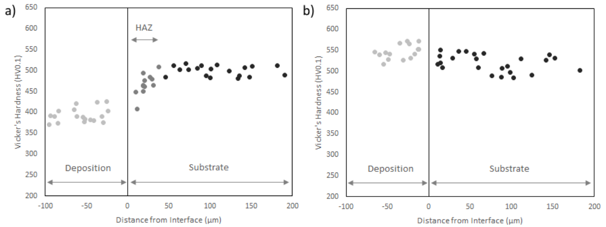
Fig. 8 Alloy 718 depositions on aged alloy 718 with a) no post-ESD heat treatment and b) with a direct aging heat treatment
